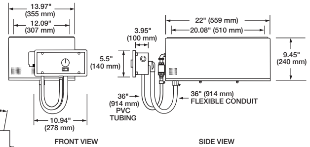
Model HWBIB-FULDA with Auto-fill Insulated Bottom Mount Series
