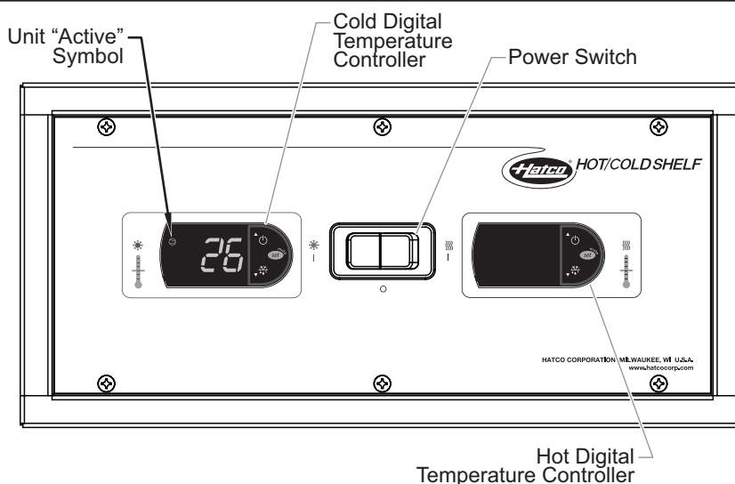
Hot/Cold Shelf Control Box (shown operating in COLD Mode)
