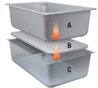
Additional Humidity A. Stainless steel food pan B. HDW-SPLASH accessory Splash baffle C. HDW-SPILL accessory Water/spillage pan (add 1/4" of water)
