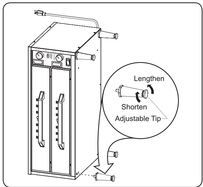
Leg Installation
