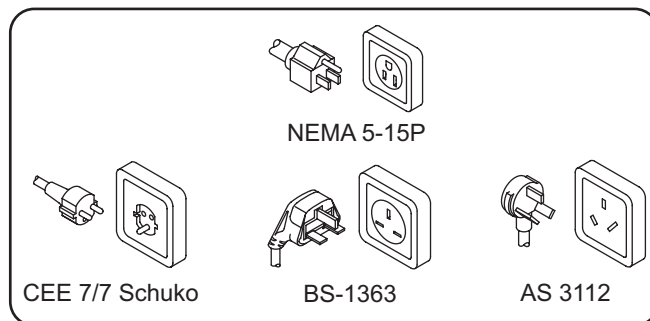
Plug Configuration
